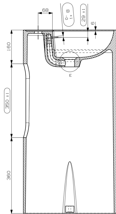
SECTION D-D SCALE 9:50
